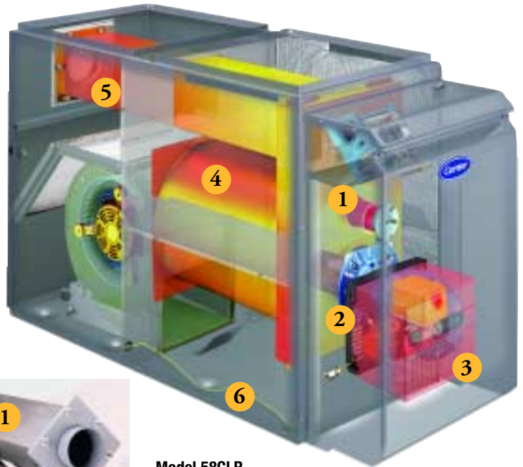
Model 58CLR Low-Boy
