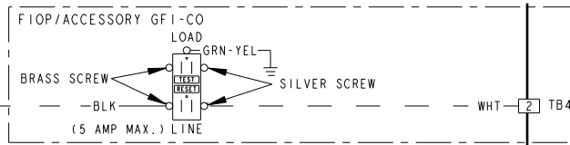
Fig. 1 — GFI-CO Location and Wiring — 30HXA,HXC076-271 Units
