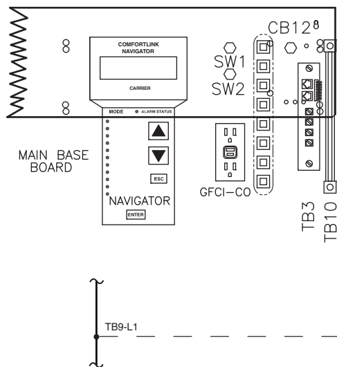
Fig. 3 — GFI-CO Location and Wiring — 30XA080-122 Units, 460/575 V
