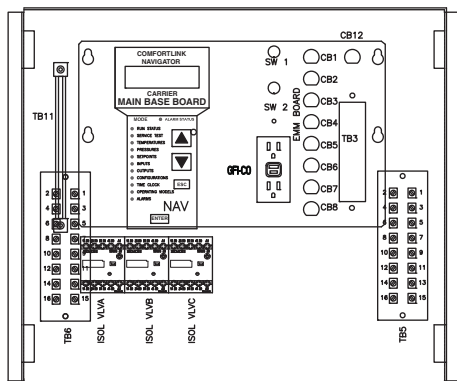
Fig. 1 — GFI-CO Location and Wiring — 30HXA,HXC076-271 Units
