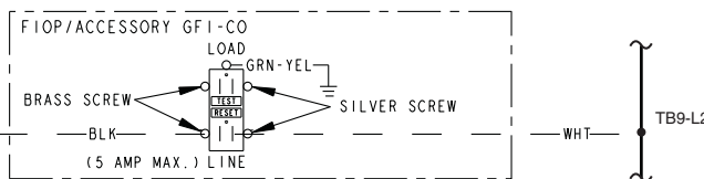
Fig. 2 — GFI-CO Location and Wiring — 30XA080-122 Units, 200/230 V and 30XA140-500 Units, All Voltages
