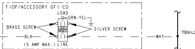
Fig. 3 — GFI-CO Location and Wiring — 30XA080-122 Units, 460/575 V
