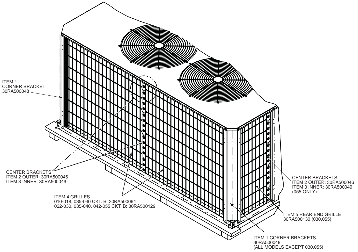
Fig. 1 — Grille Option and Components
