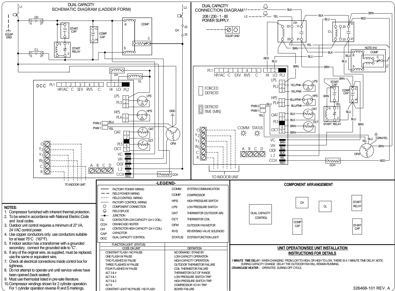
Fig. 2—Wiring Diagram—037
