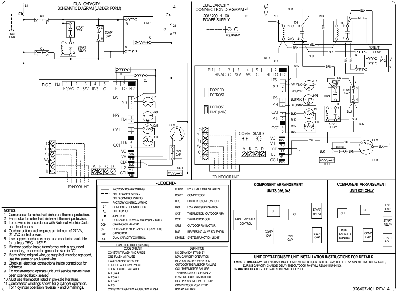
Fig. 1—Wiring Diagram—024, 036, 048
