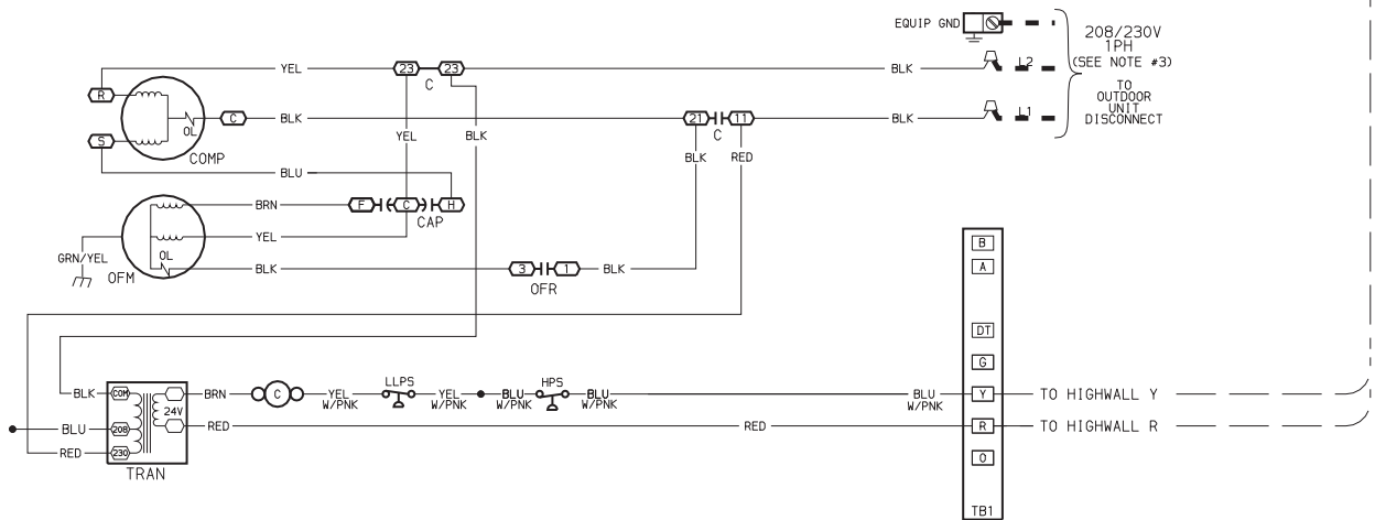
Fig. 13 – 40QNC01824 Matched with 38HDF Typical Wiring Schematic
