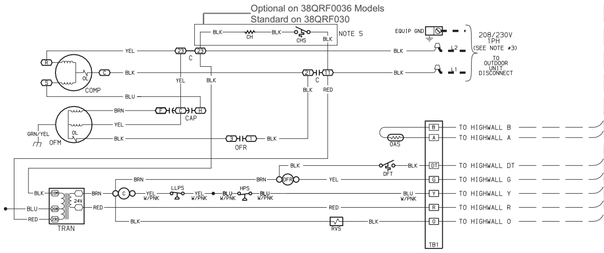
Fig. 16 - 40QNQ030,036 Matched with 38QRF Typical Wiring Schematic
