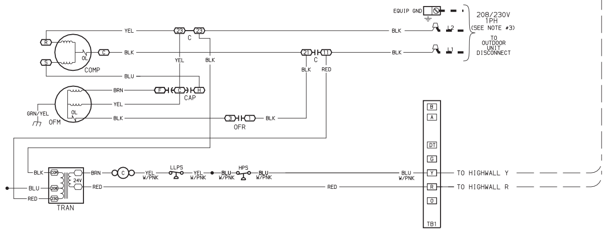
Fig. 15 - 40QNC030,036 Matched with 38HDF Typical Wiring Schematic
