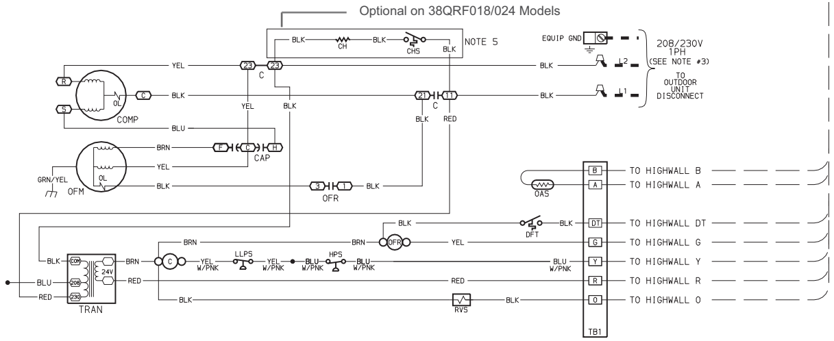
Fig. 14 – 40QNQ018,024 Matched with 38QRF Typical Wiring Schematic
