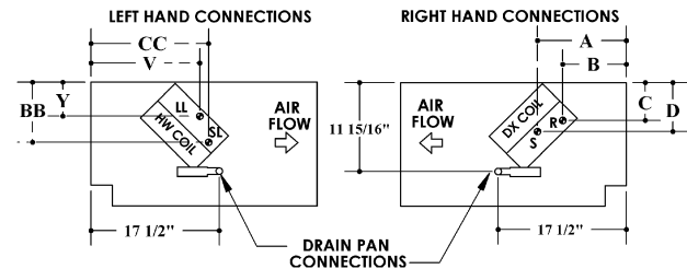
HW/DX 4-pipe
