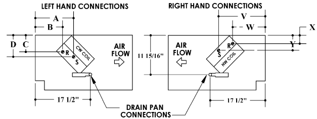
HW/CW 4-pipe
