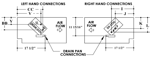
Steam/DX 4-pipe
