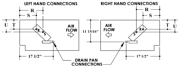
HW/CW 2-pipe
