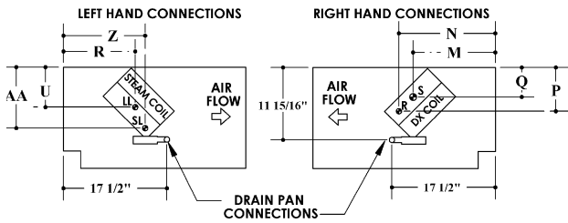
DX/Steam 4-pipe
