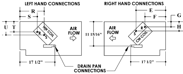
CW/HW 4-pipe
