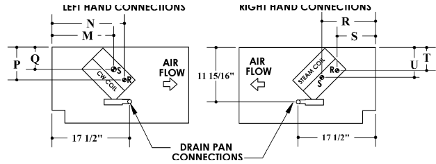
CW/Steam 4-pipe
