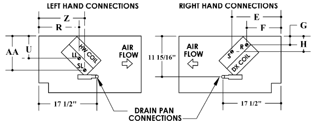
DX/HW 4-pipe
