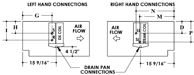
Steam/DX 4-pipe
