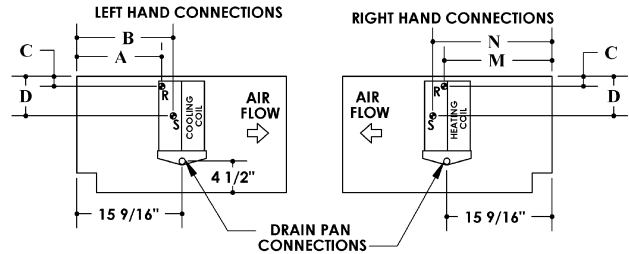
HW/CW 4-pipe
