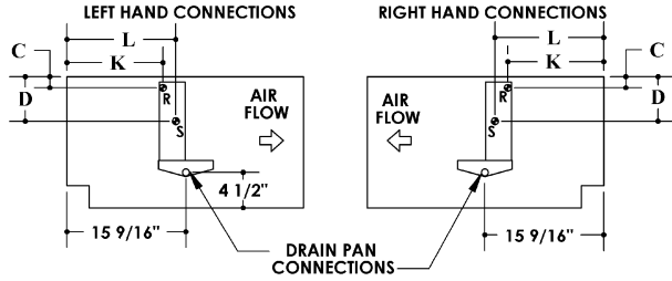
HW/CW 2-pipe
