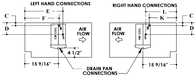
CW/HW 4-pipe
