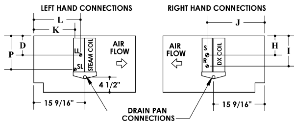
DX/Steam 4-pipe
