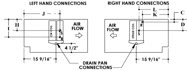
CW/Steam 4-pipe
