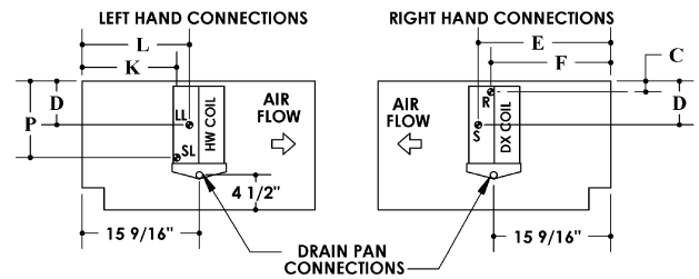
DX/HW 4-pipe
