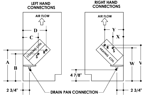
HW/CW 4-pipe
