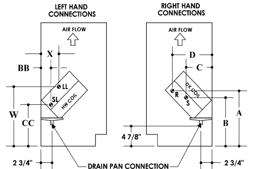
HW/DX 4-pipe
