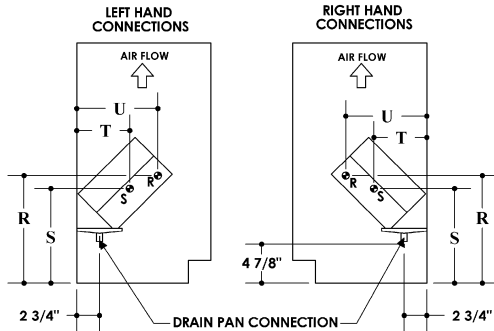
HW/CW 2-pipe
