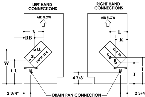
Steam/DX 4-pipe
