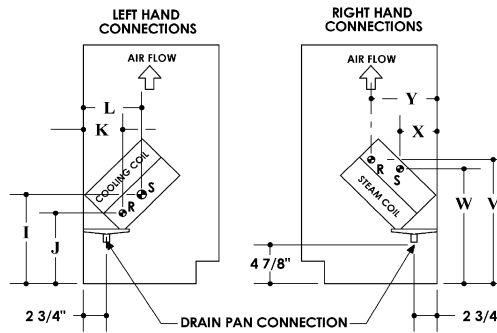
Steam/CW 4-pipe
