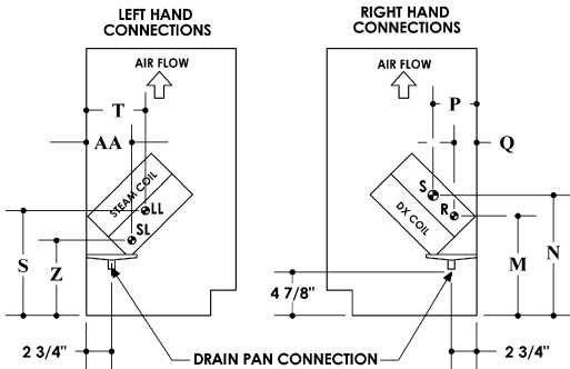
DX/Steam 4-pipe
