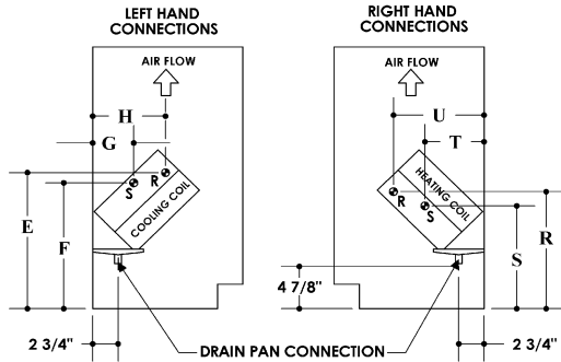
CW/HW 4-pipe
