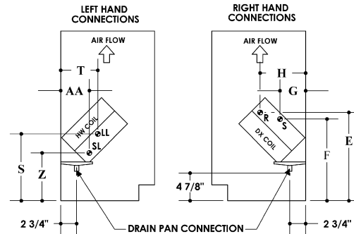
DX/HW 4-pipe
