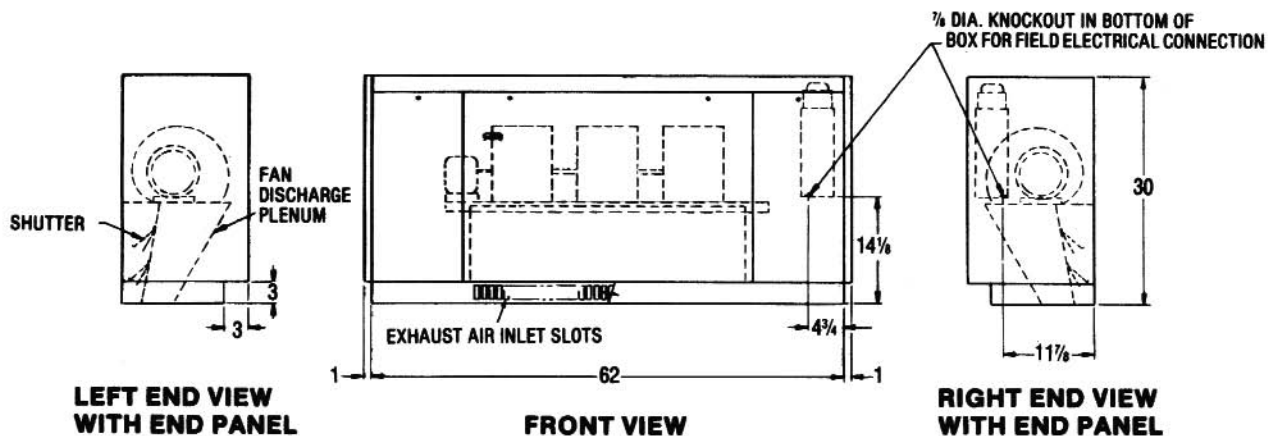
FRONT VIEW
