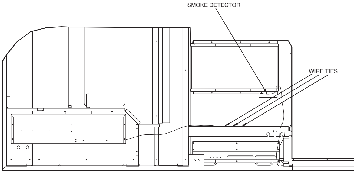
Fig. 9 – Supply Smoke Detector Location and Wire Routing (Top View)
