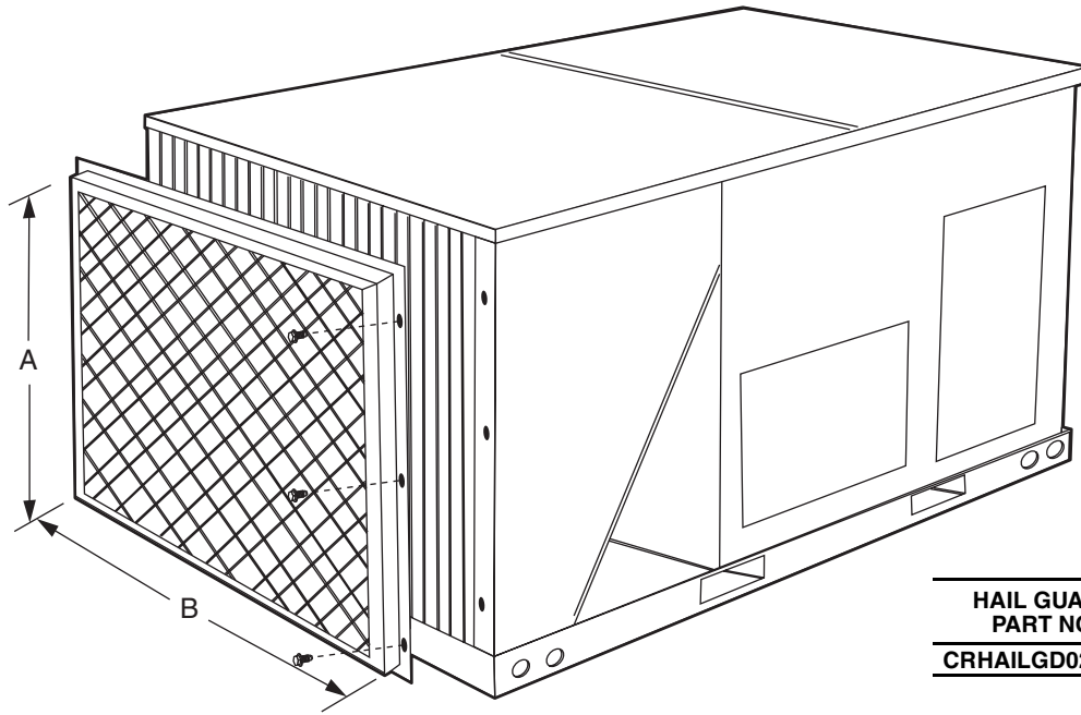
Fig. 1 — Hail Guard Installation
