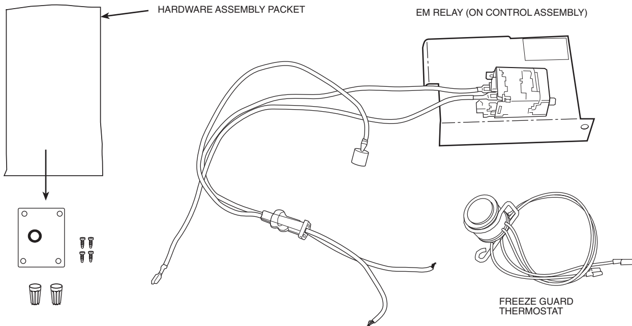
Fig. 1 — Energy Management (EM) Accessory Kit
