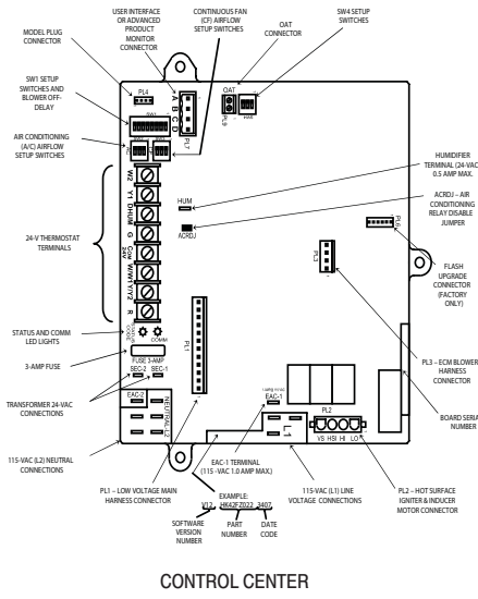
CONTROL CENTER
