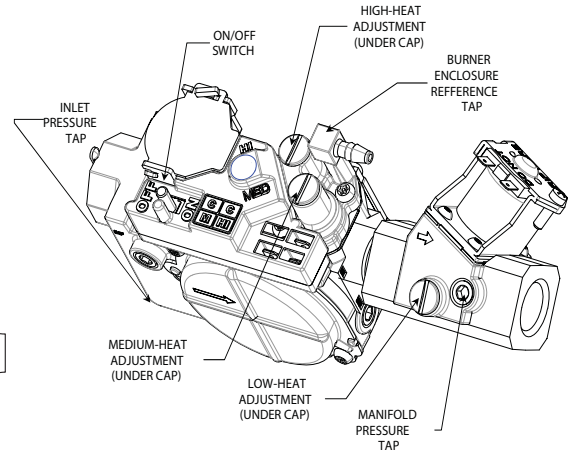
GAS VALVE
