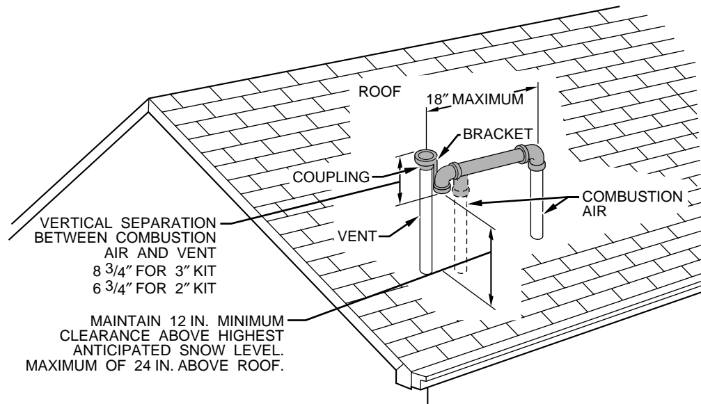
Fig. 3— Roof Termination (Preferred)
