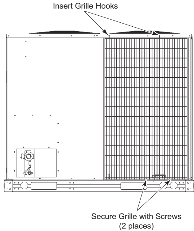
Fig. 2 - 38AU with Outside Coil Grille - Right Side View
