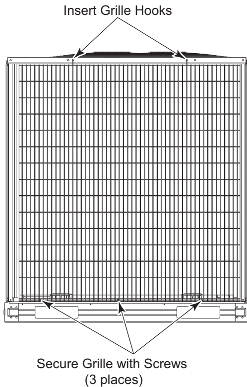
Fig. 1 - 38AU with Outside Coil Grille - Back View
