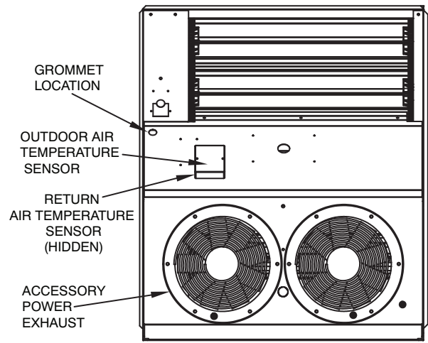
Facing Economizer
