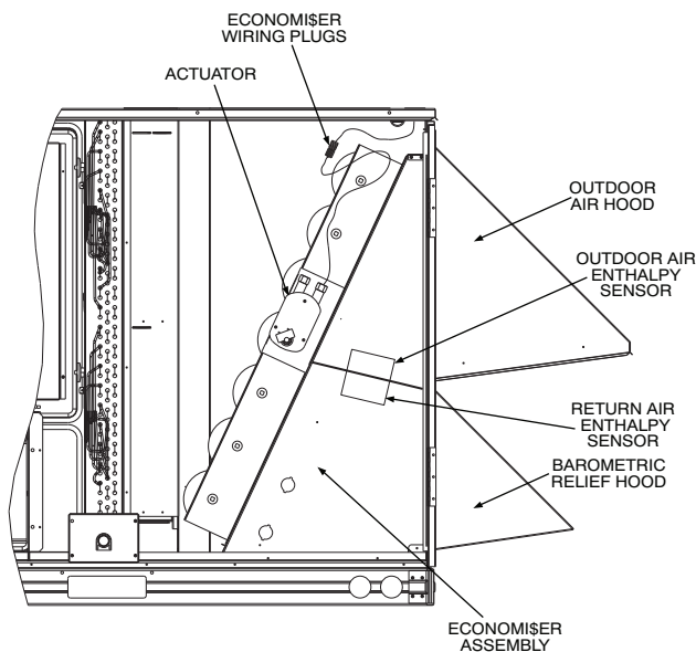
Fig. 1 - Side View of Vertical Economi$er — 48/50PD05-06 and 48/50PG03-16 Units
