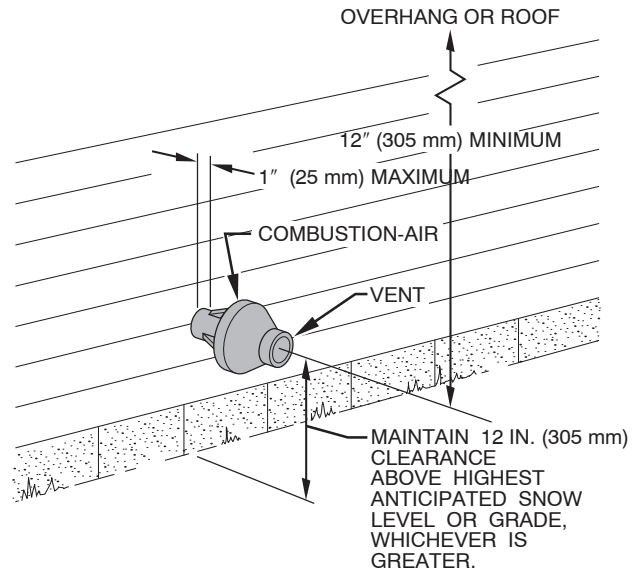
Fig. 6 - Concentric Vent and Combustion-Air Side Wall Termination
