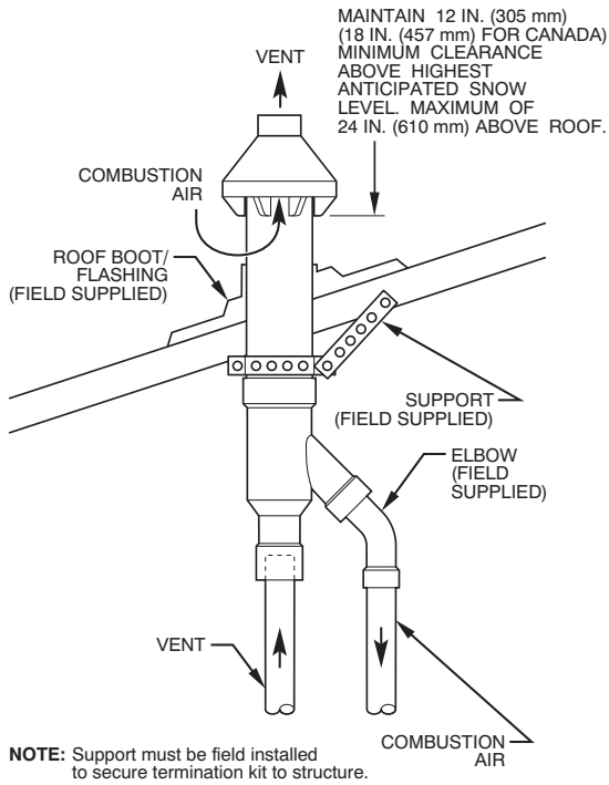
Fig. 5 - Concentric Vent Roof Installation
