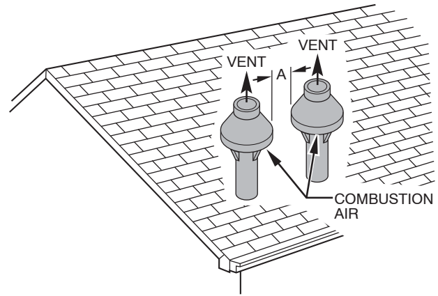
Fig. 8 - Concentric Vent and Combustion-Air Roof Termination (Dimension A as Touching or 2-in. (51 mm) Maximum Separation)
