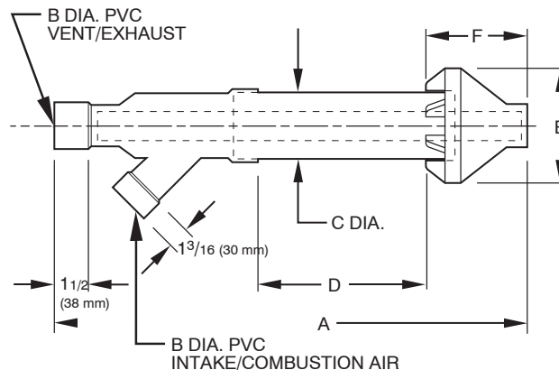
Fig. 2 - Concentric Vent Dimensional Drawing
