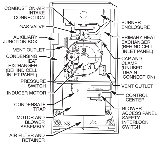
Fig. 1 - Component Location in 40-in. (1016 mm) Tall Condensing Furnace (Upflow Orientation Shown)
